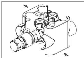
Illustr. 8 Installation of the straight pattern design cover
