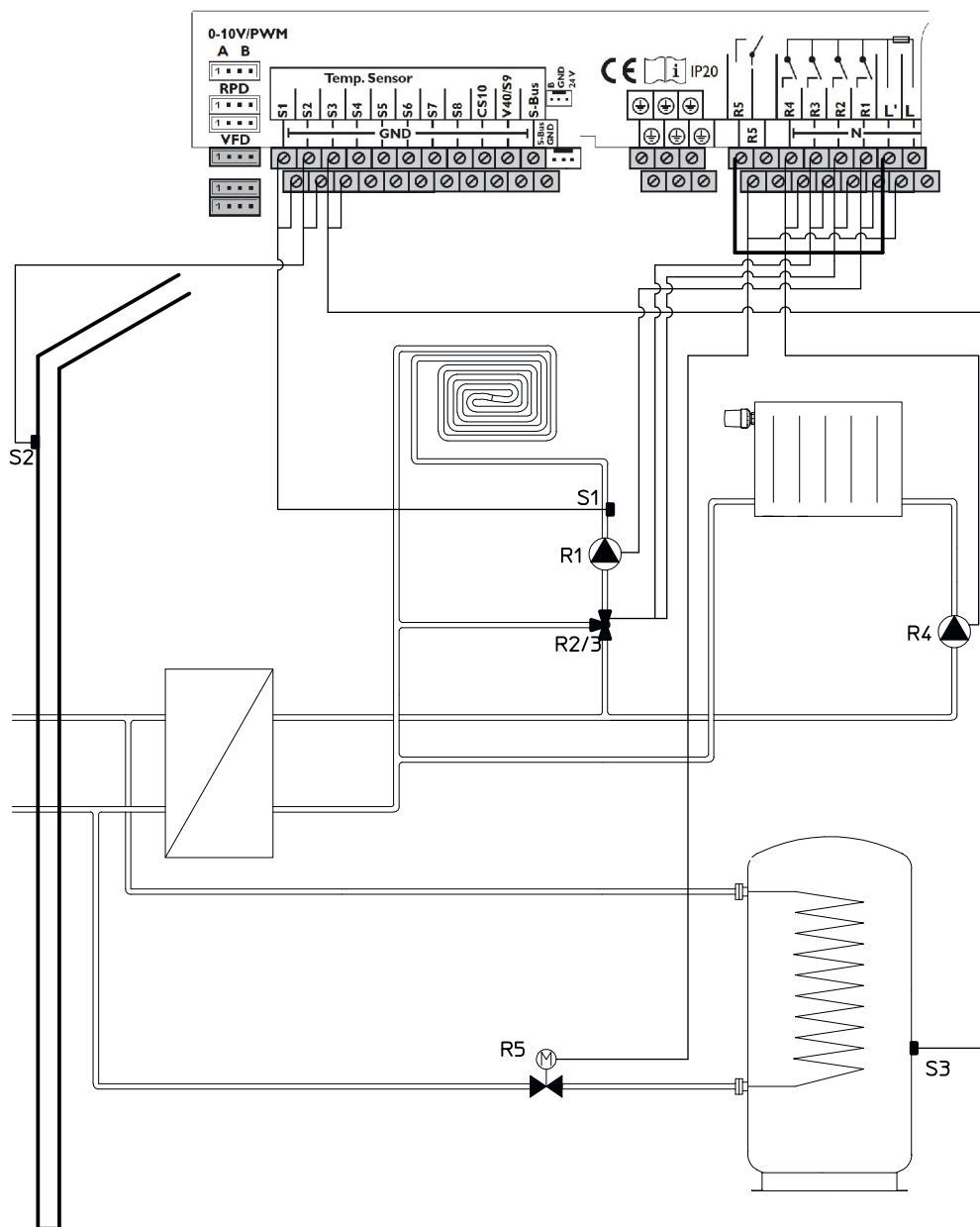
Illust. 53: Scheme 6, one variable and one constant temperature heating circuit, direct hot potable water preparation
