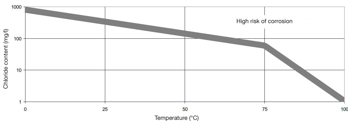
Premissible chloride content depending on the temperature
