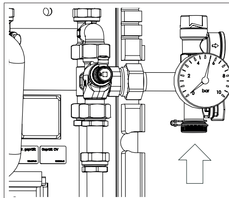
Illust. 43: Fill and drain ball valve of the safety group
