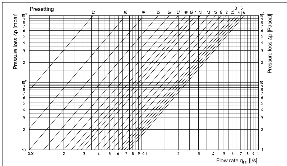
Illustr.. 9.1: Chart of double regulating and commissioning valve "Hycoco VTZ" DN 20
