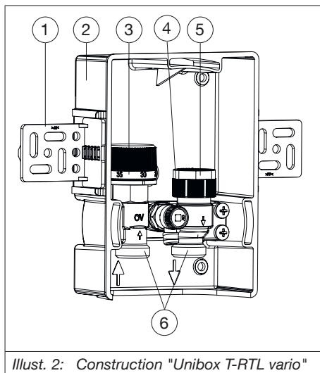
Illust. 2: Construction "Unibox T-RTL vario"
