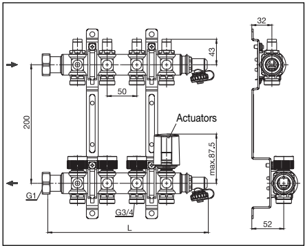
Illustr. 1: Dimensions
