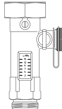
Illustr. 5: Flow measuring and regulating device, OV item no. 136 41 60/61/62
