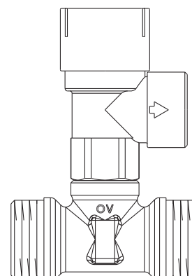
Illustr. 7: Safety valve 6 bar, OV item no. 136 41 10
