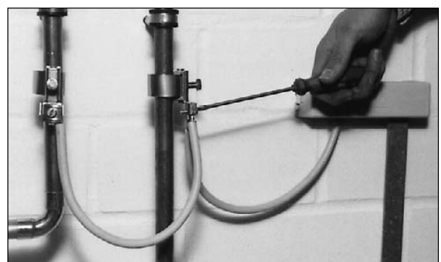
Illustr. 9: For equipotential bonding, fix earth clips onto both solar circuit pipes and connect a cable with a minimum section of 6 mm 2 to the main equipotential bonding rail.
