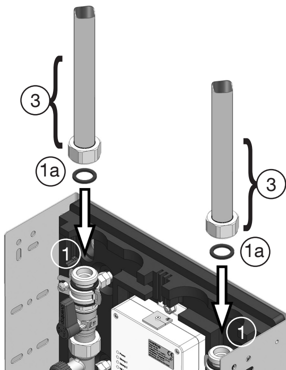
Illustr. 31: "Regudrain Duo" in a serial installation
