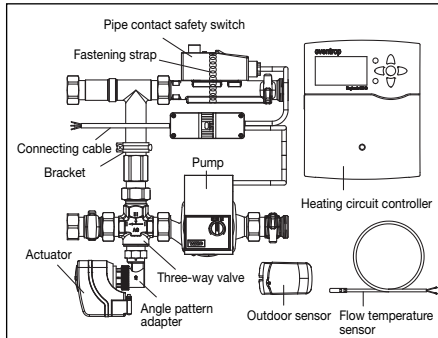
Illustr. 5.1 Summary "Regufloor HW"
