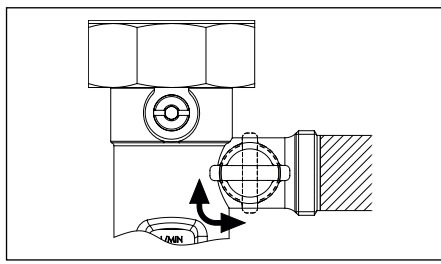
Illustr. 6.18 Bleeding via the flow measuring and regulating device
