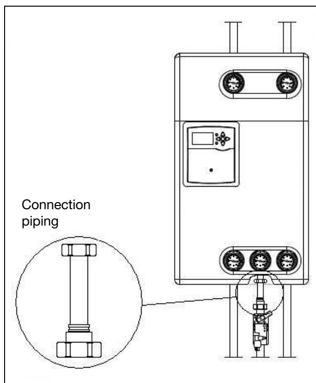
Connection piping 1389082 Installation example
