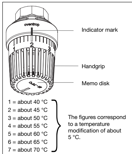
Illustr. 7.2: Temperature controller
