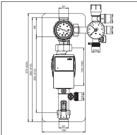
Illustr. 4.1 Pump circuit "Regusol PH-130 (180)" DN25 16
