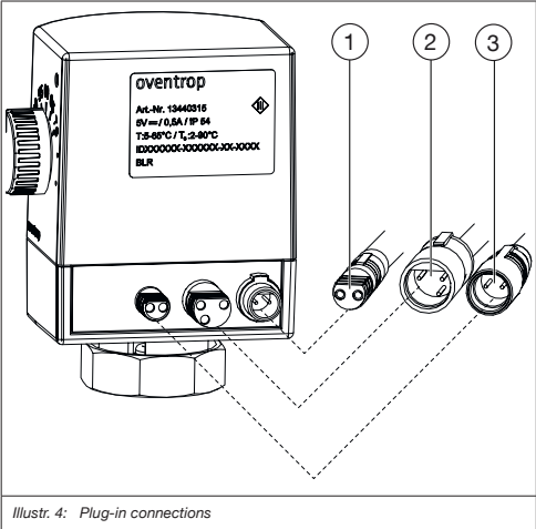
Illustr. 4: Plug-in connections
