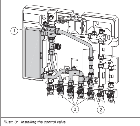
Illustr. 3: Installing the control valve
