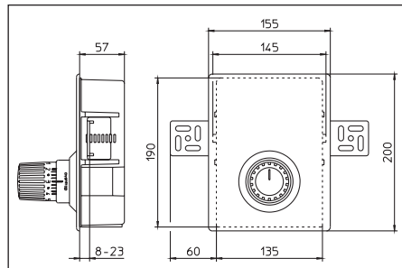
Illustr. 4.1 Dimensions
