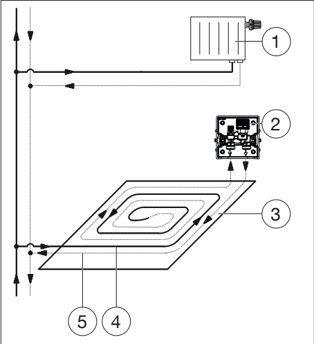
Fig. 6: Raccordement
