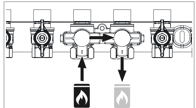
Illustr. 4: Flow direction "Flypass" fitting flushing
