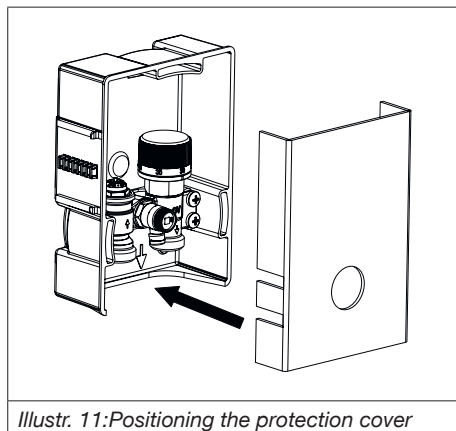
Illustr. 11: Positioning the protection cover
