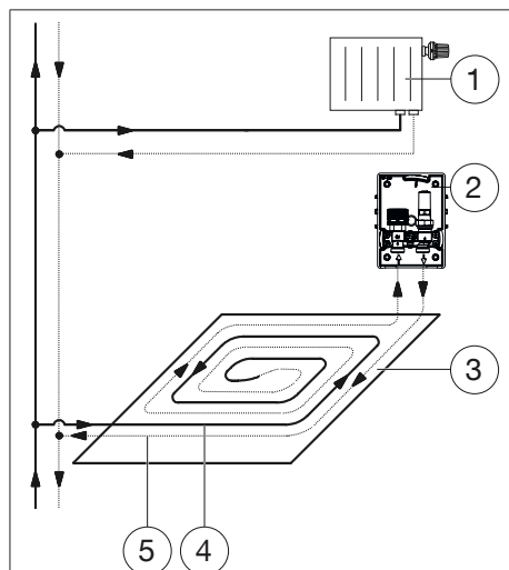
Fig. 9: Raccordement
