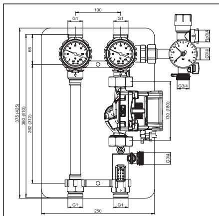
Abb. 4.2 Solarstation „Regusol SH-130 (180)“ DN 25
