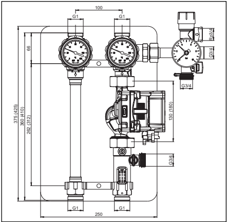
Illustr. 4.2 Solar station "Regusol SH-130 (180)" DN25
