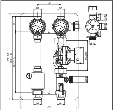
Illustr. 4.3 Solar station "Regusol LH-130 (180)" DN25
