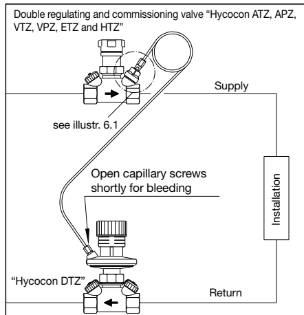
Illustr. 6.2: "Hycoco DTZ", installation in the return pipe
