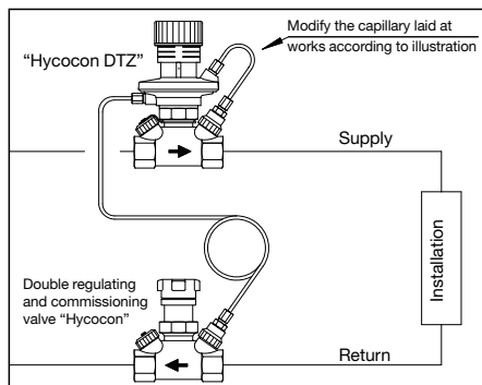
Illustr. 6.3: "Hycoco DTZ", installation in the supply pipe (only DN 32 + 40)
