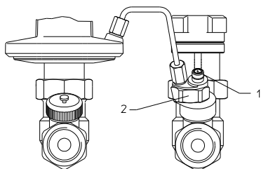
Illustr. 6.1: "Hycoco DTZ", capillary connection, installation
