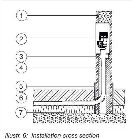
Illustr. 6: Installation cross section
