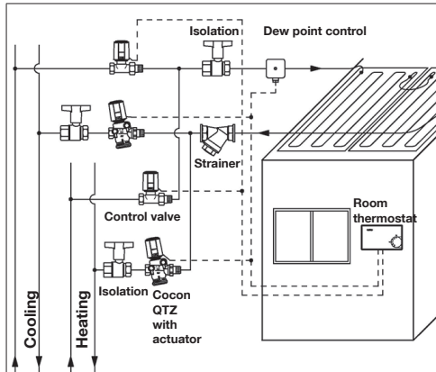
Fig. 7: Installation example 2: Four pipe system
